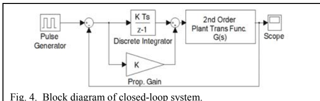
Fig. 4. Block diagram of closed-loop system.
