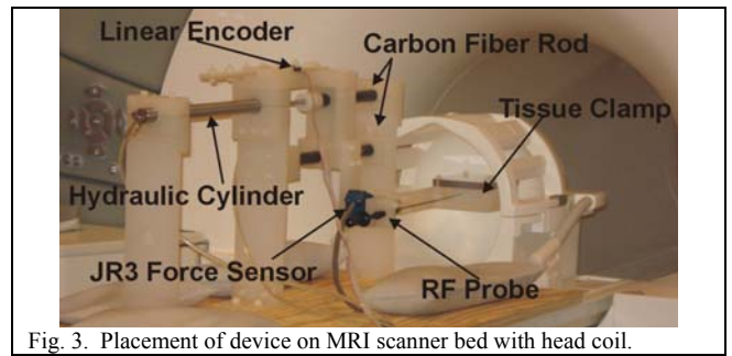
Fig. 3. Placement of device on MRI scanner bed with head coil.
