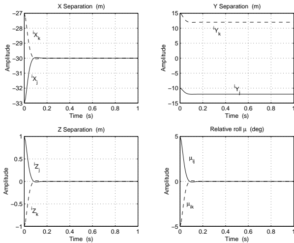
Figure 4: Controlled output variables of follower UAVs.
