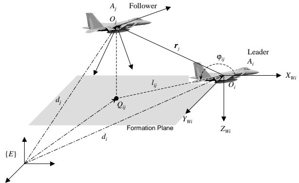
Figure 2: Flight formation geometry.
